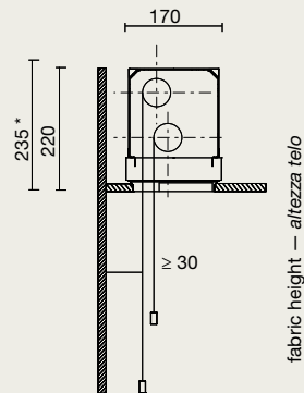
Lowering of the fabrics: in front of both rollers (standard) Discesa dei teli: avanti (standard)
