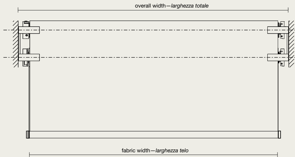
Front view Vista frontale
