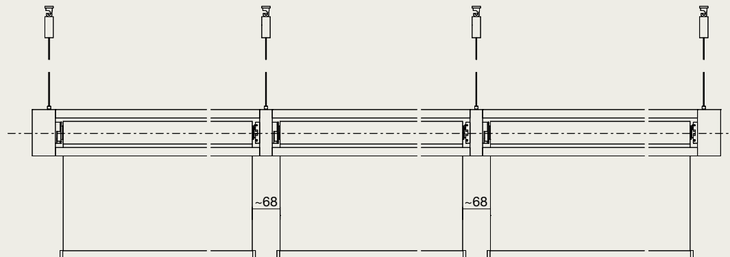
Front view Vista frontale
