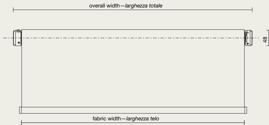
Front view Vista frontale
