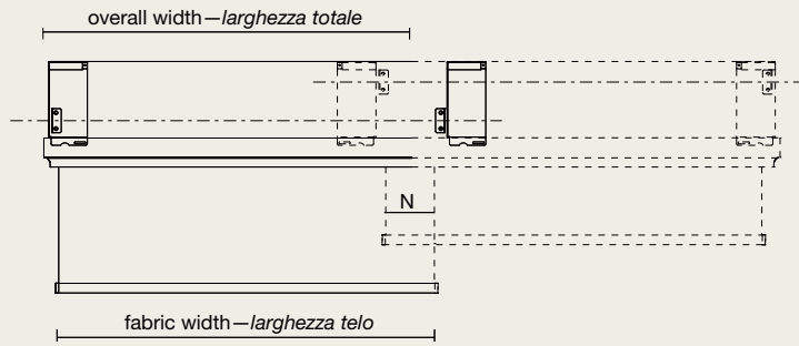
Front view Vista frontale
