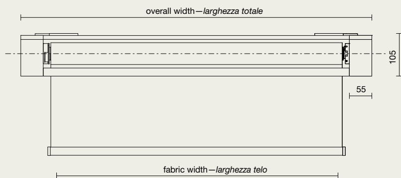
Front view Vista frontale
